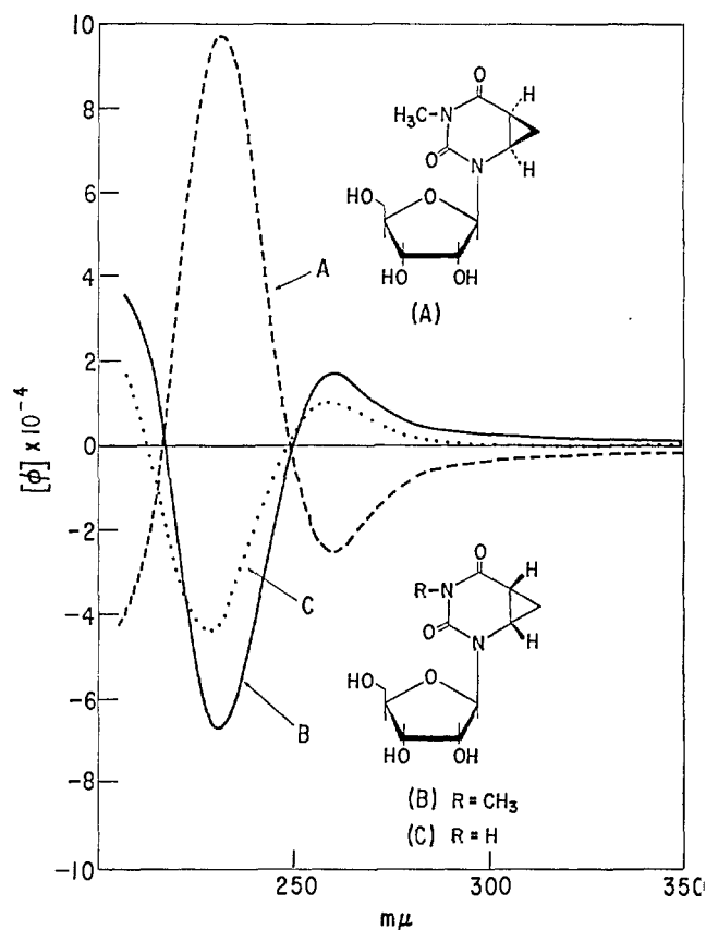
Figure 1. ORD curves of 1- \beta -D-ribofuranosyl-3-methyl-5,6 \alpha -cyclothymines (A) and 5,6- \beta -cyclothymines (B) and of 1- \beta -D-ribofuranosyl-5,6 \beta -cyclothymines (C) in H 2 O.
